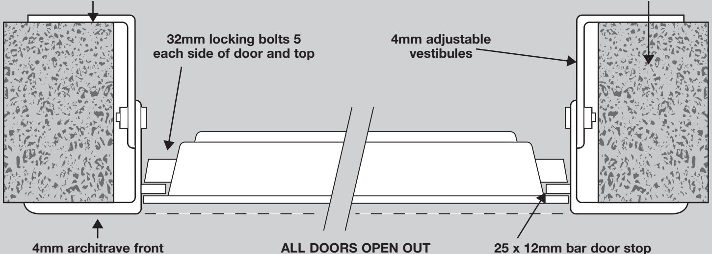
Adjustable 10mm thick fixing plate
